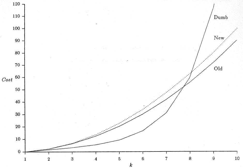
Figure 9. Total experimental cost for n=2^k-1 , k=2..9
