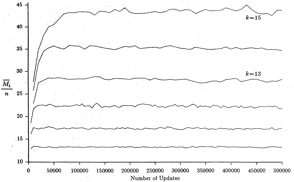
Figure 4b. Simulation results for n=2^k-1 , k=10..15 .
