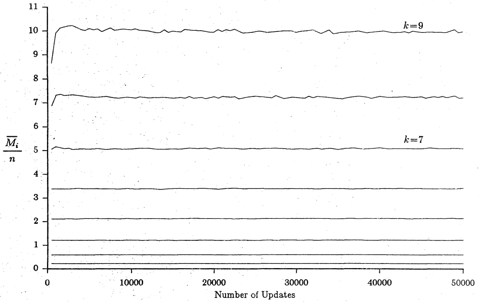
Figure 4a. Simulation results for n=2^k-1 , k=2..9 .
