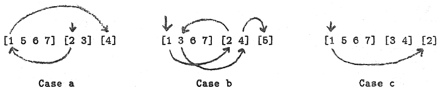
Figure 7: Examples of optimal sequences of replacements.
