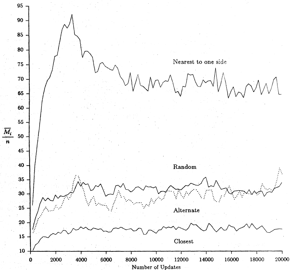
Figure 1. Simulation results for different heuristics ( n=2047 ).
