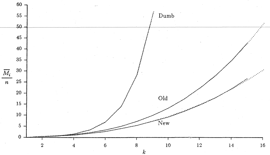
Figure 6. Asymptotic simulation results for n=2^k-1 , k=2..15
