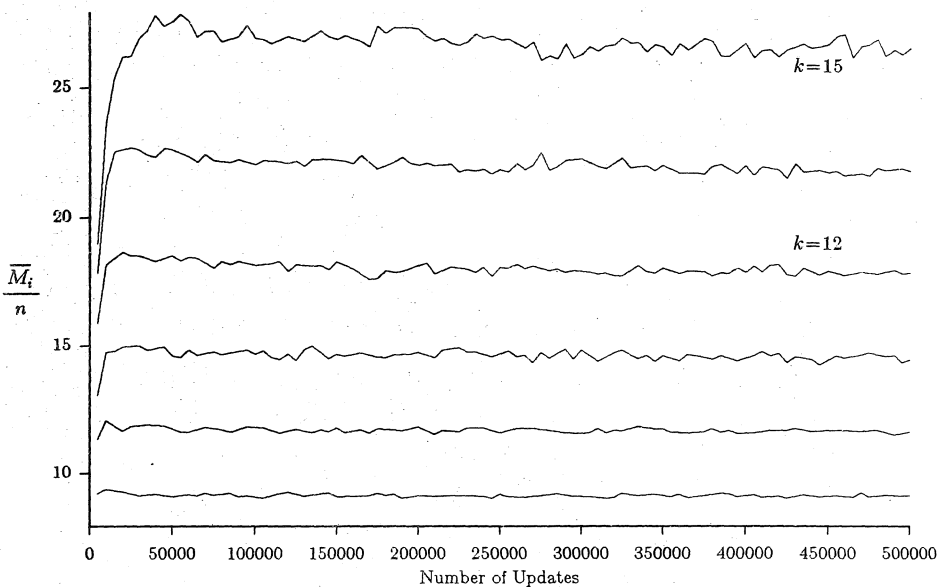
Figure 8b. Simulation results (new algorithm) for n=2^k-1 , k=10..15
