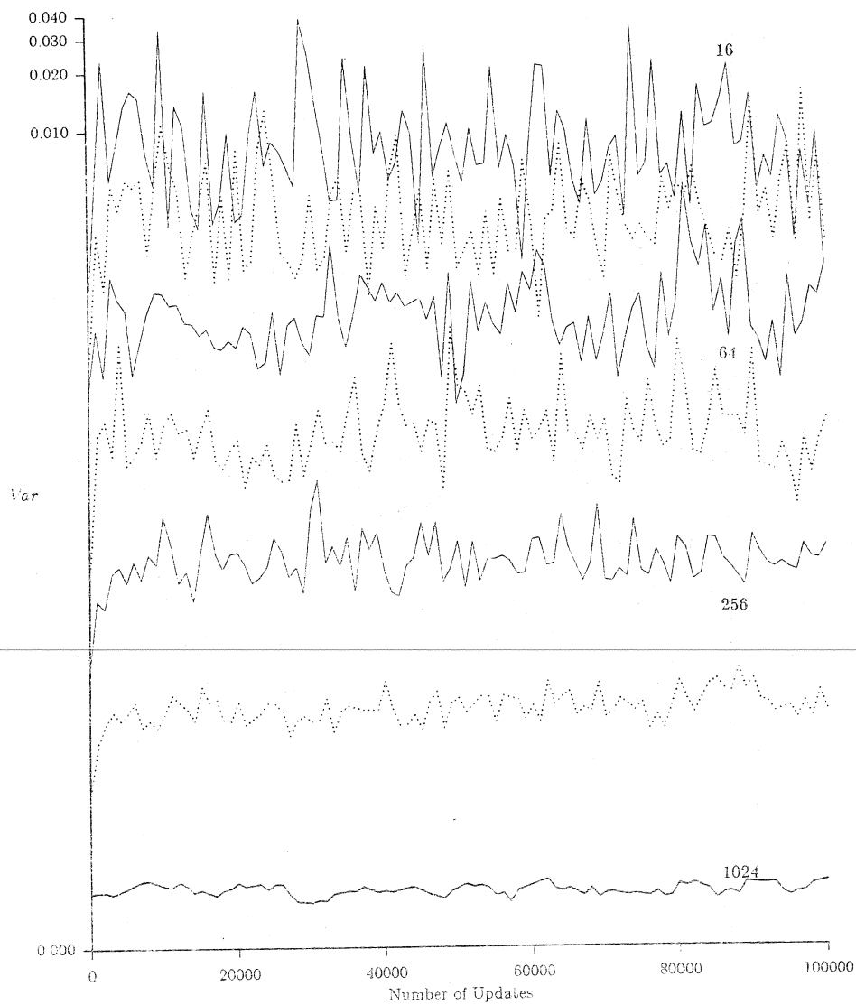
Figure 2. Simulation results for the variance on each list for n=2047 .
