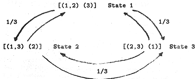
Figure 3: Markov chain for n = 3 .
