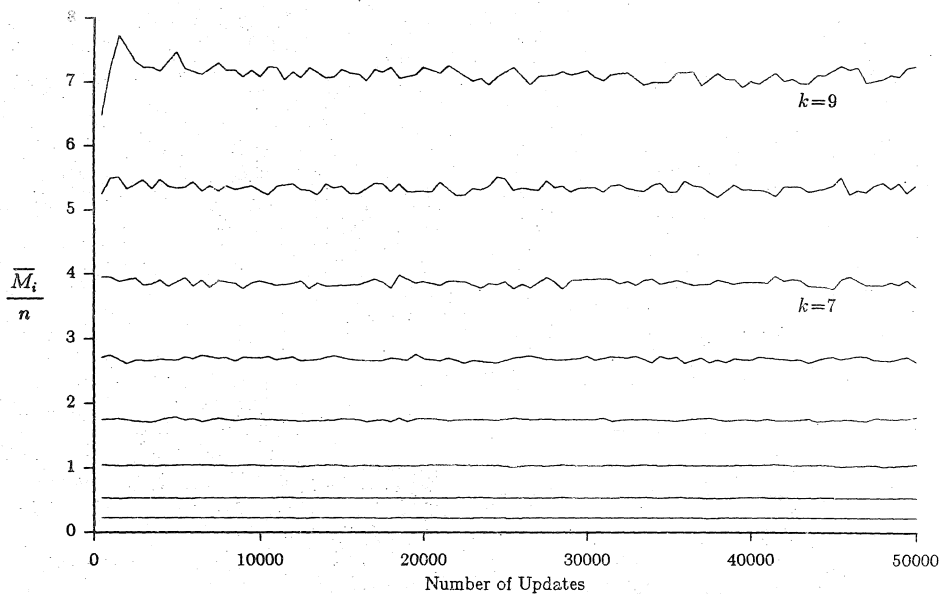
Figure 8a. Simulation results (new algorithm) for n=2^k-1 , k=2..9
