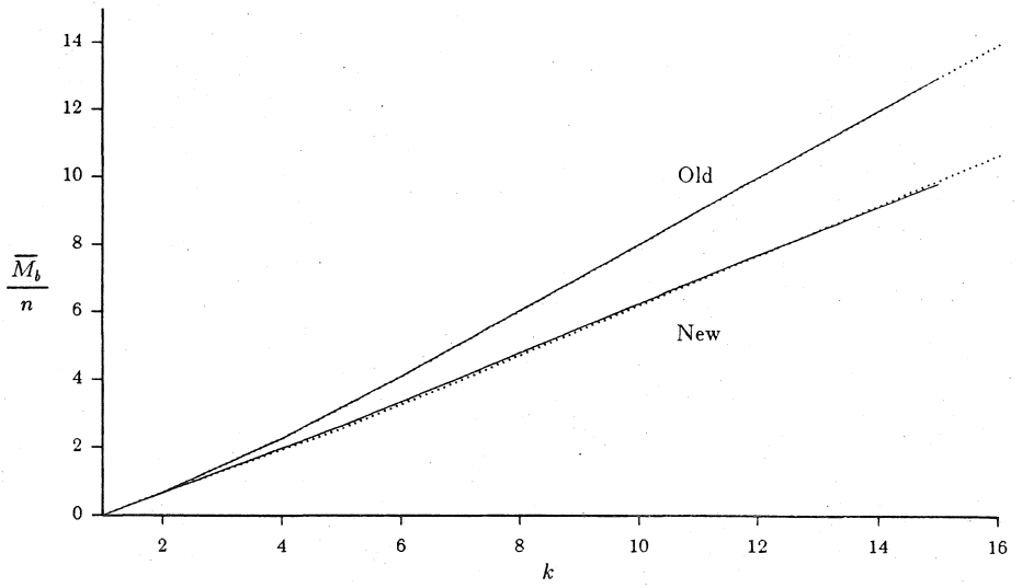
Figure 5. Asymptotic simulation results for n=2^k-1 , k=2..15
